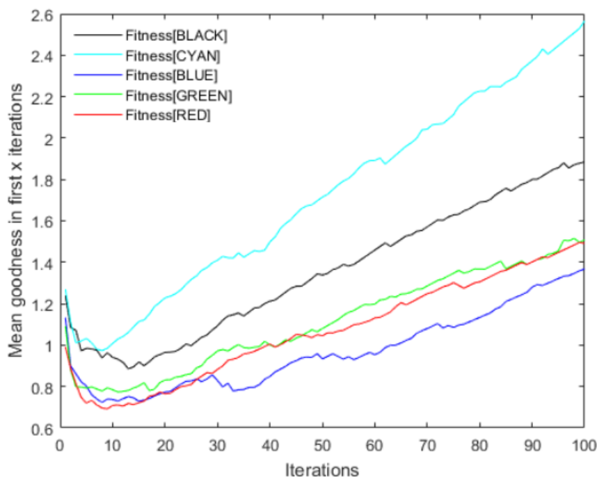
Figure 5: Average goodness of fitness functions in long-text examples
